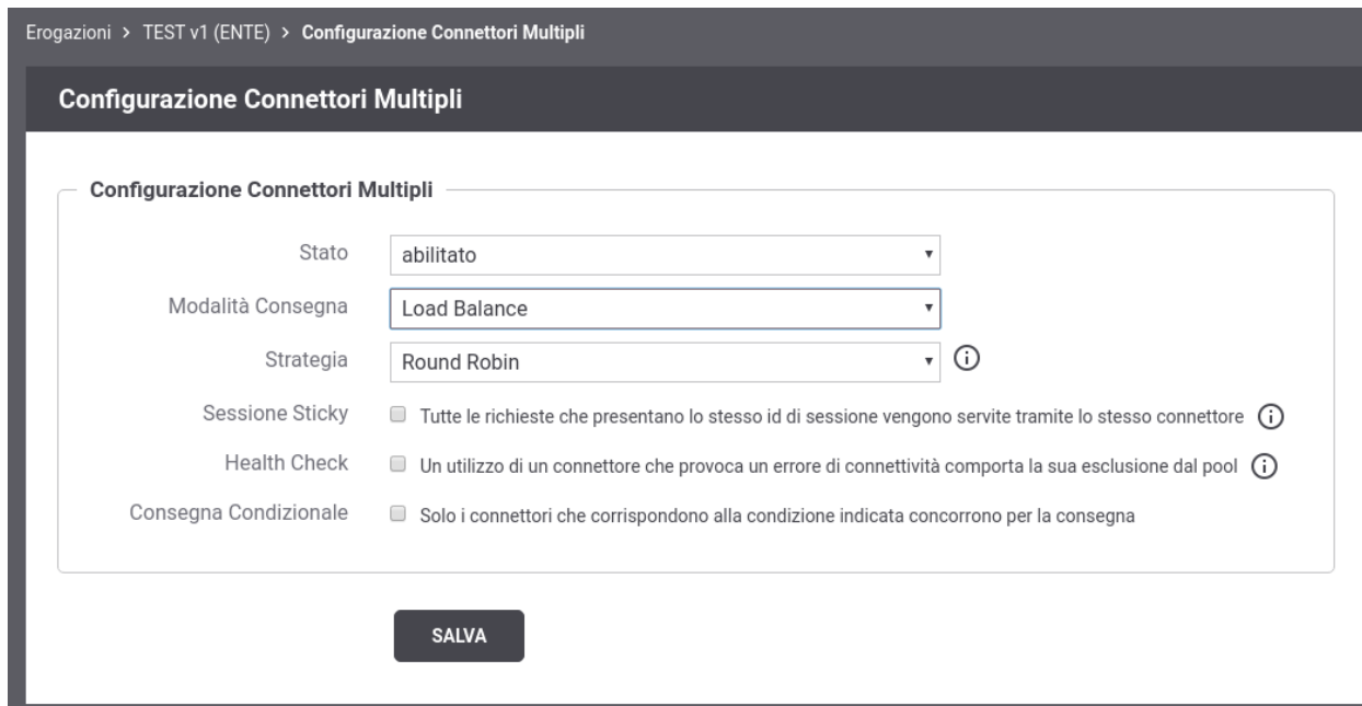
Fig. 2.29: Load Balancer
